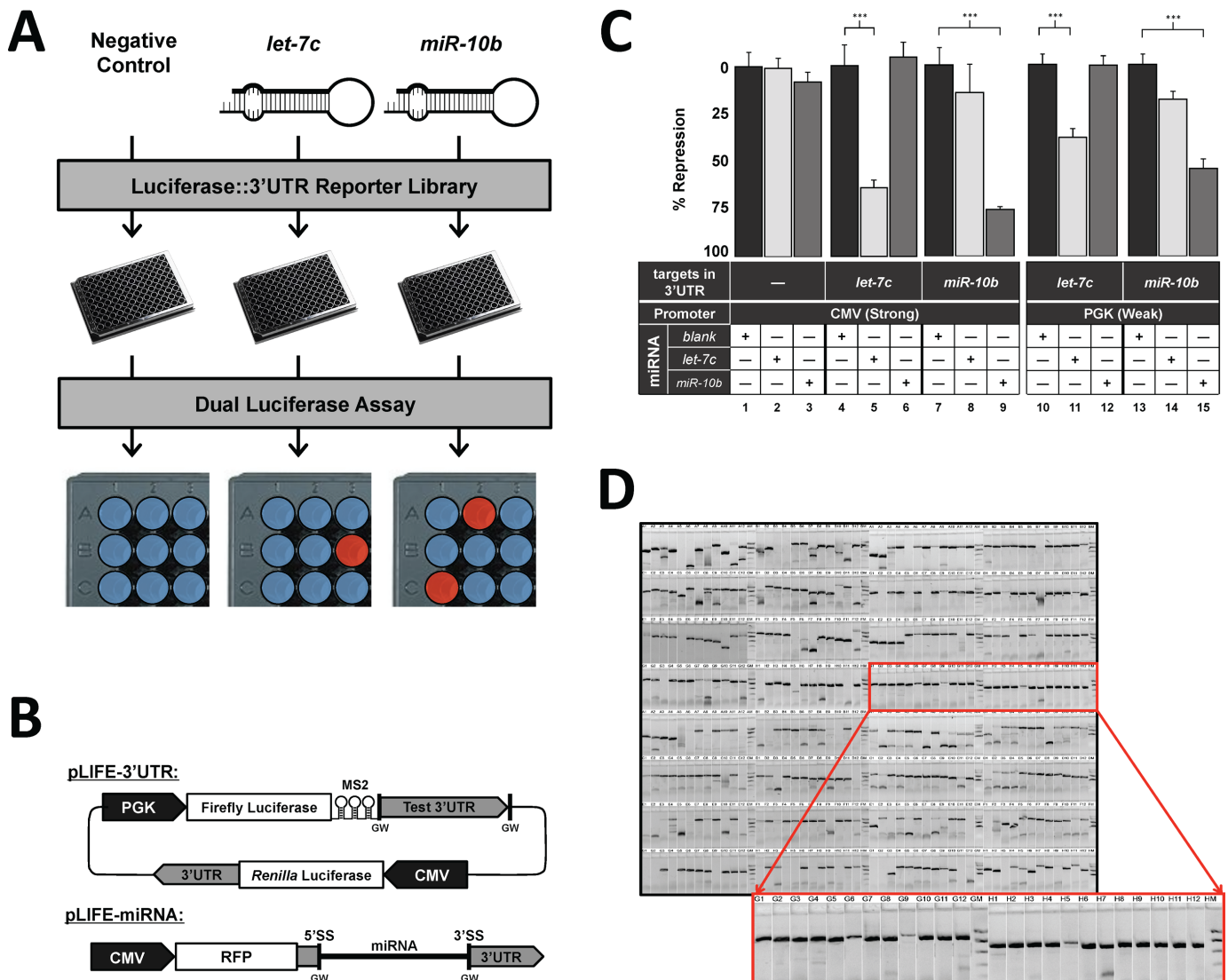
Figure 1. The 3'LIFE Assay. (A) Schematic of the 3'LIFE assay. A reporter library of luciferase::3'UTR fusion genes is cotransfected in HEK293T cells with miRNAs of interest and a negative control in 96-well format. Following transfection cell lysate is used in a dual luciferase assay, and target genes are identified by a significant repression of the luciferase gene compared to the negative control (B) 3'LIFE Vector Design. (Top) Gateway compatible dual luciferase expression vector. The 3'UTR of interest is cloned downstream of firefly luciferase using Gateway cloning. Both luciferase genes are located on the same plasmid to prevent fluctuations in the luciferase ratio across experiments. (Bottom) Gateway compatible miRNA expression plasmid. The miRNA of interest is cloned within an intron in the 3'UTR of RFP using Gateway cloning. This approach functions dually as a visual marker for transfection efficiency and miRNA expression. (C) Positive controls for let-7c and miR-10b . The SV40 3'UTR containing a scrambled miR-10b target site (blank) or let-7c and miR-10b targets were cloned into the pLIFE-3'UTR and tested in quadruplicate using a dual luciferase assay. Results are normalized to the Blank condition of each 3'UTR. Y-axis measures the percentage of repression compared to the Blank condition. Error bars are standard error unless otherwise noted. * denotes statistical significance (Student's t -test, * P < 0.05 , ** P < 0.01 and *** P < 0.001 ). (D) Gel electrophoresis of 384 3'UTRs amplified from human genomic DNA using touchdown PCR for use in the 3'LIFE assay.
