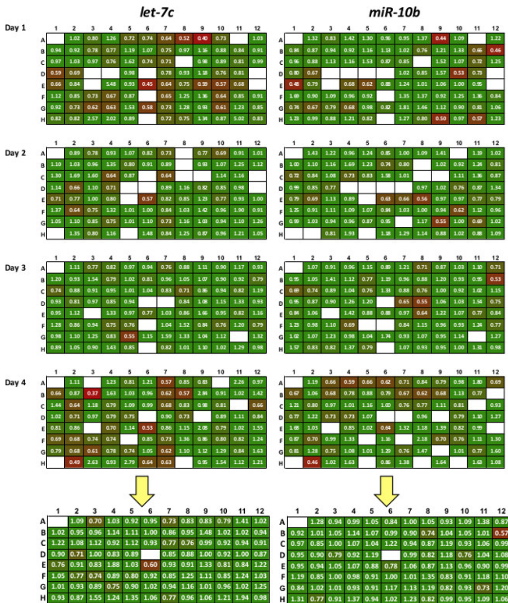
Figure 2: Sample of data produced with 3'LIFE assay. Each probe miRNA is tested in quadruplicate (replicates 1-4). Colors represent repression levels, with red colors indicating strong miRNA/3'UTR interaction. All replicates are averaged to produce high-quality putative targets shown in the summary plate below the yellow arrow. White box represent controls, failed transfections or wells with low transfection efficiency.
